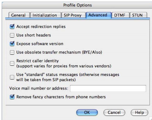
Fig.6 - Advanced
