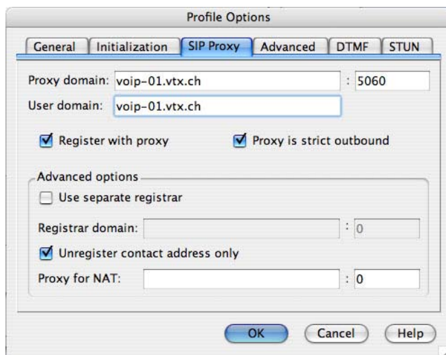
Fig.5 – SIP Proxy
